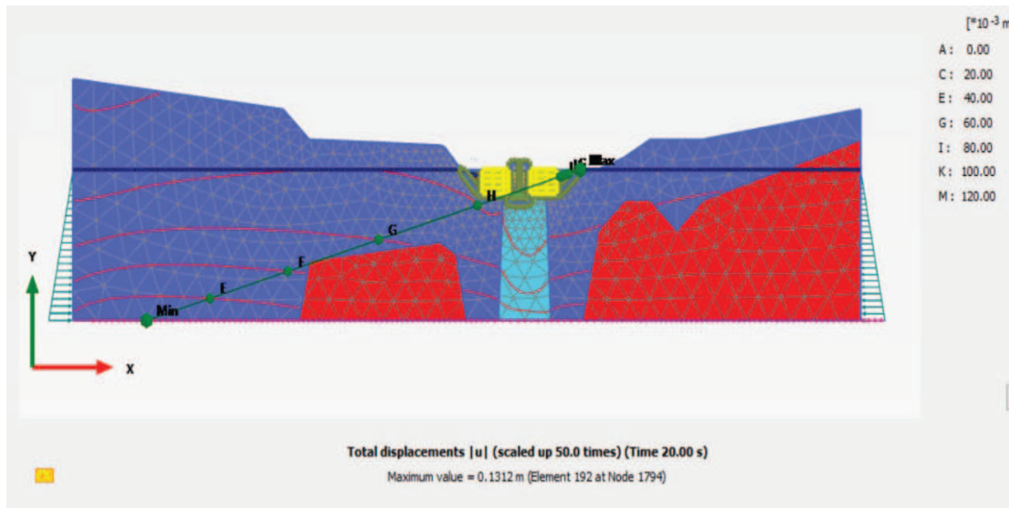
Figure 10. Total displacement in Outlet structure model due to Gorkha EQ
