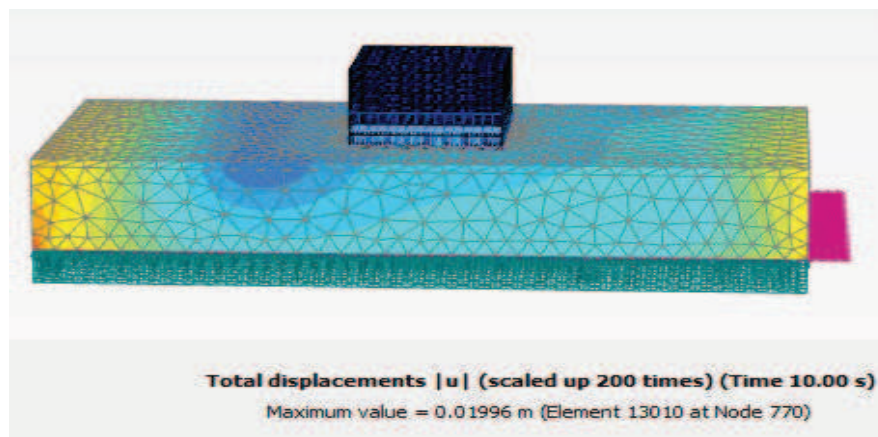
Figure 9. Total displacement in the structure
