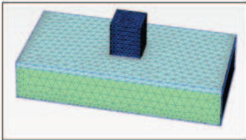
Figure 7. Generated mesh
