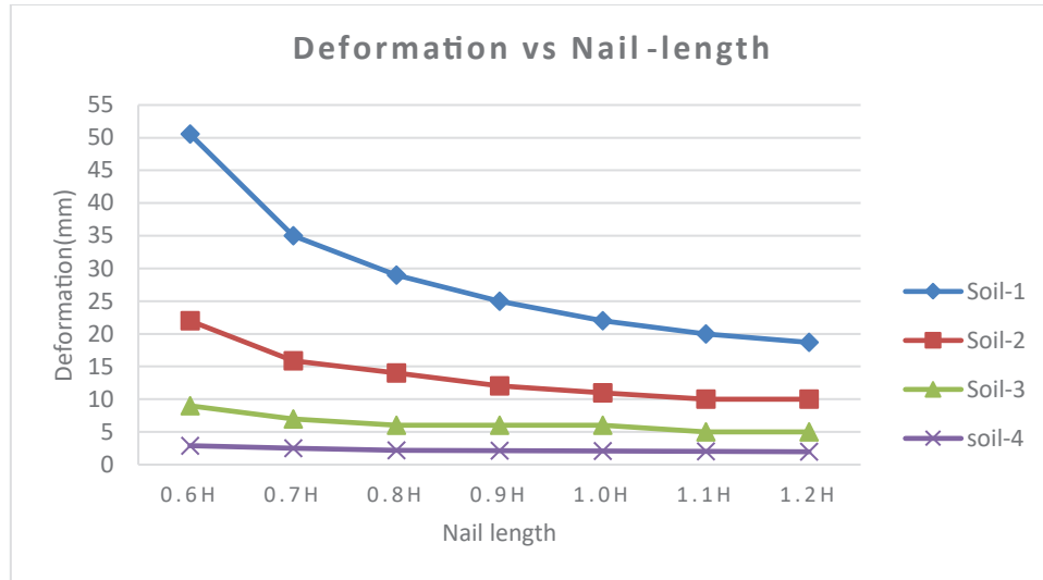
Figure 3. Effect of nail length on deformation
