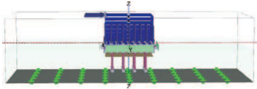
Figure 6. Structural model
