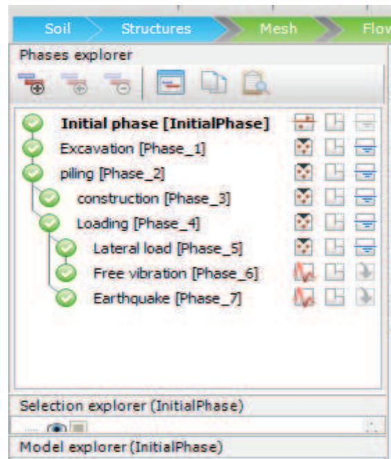
Figure 8. Stage construction
