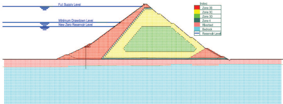
Figure 1. Geometric Model of Naumure Multipurpose Dam
