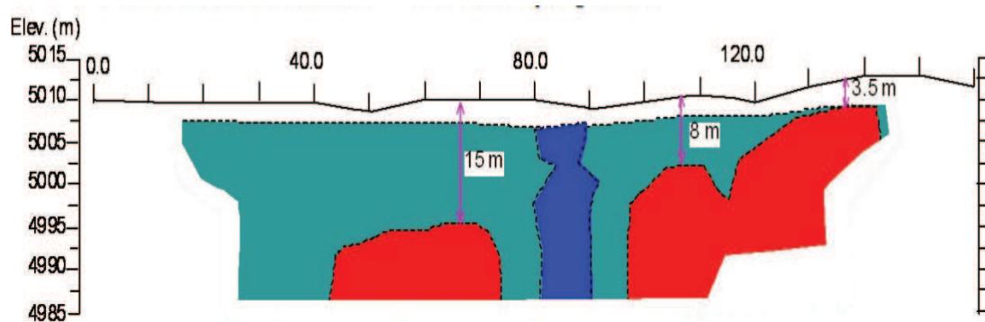
Figure 3. Geological cross-section interpreted from the geo-electric section
